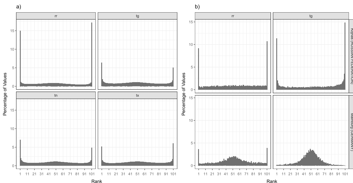
Figure 3. Rank histograms calculated for the E-OBS v16.0e ensemble compared to the 100 withheld stations, across all stations over the period 1971–2000 (a) and for two selected stations (b) over that period.
