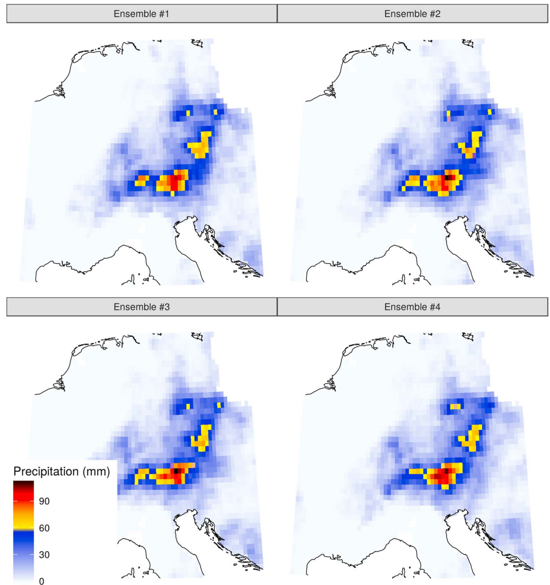
Figure 7. The first four ensemble members from E-OBS v16.0e for the precipitation event of 1 June 2013.
