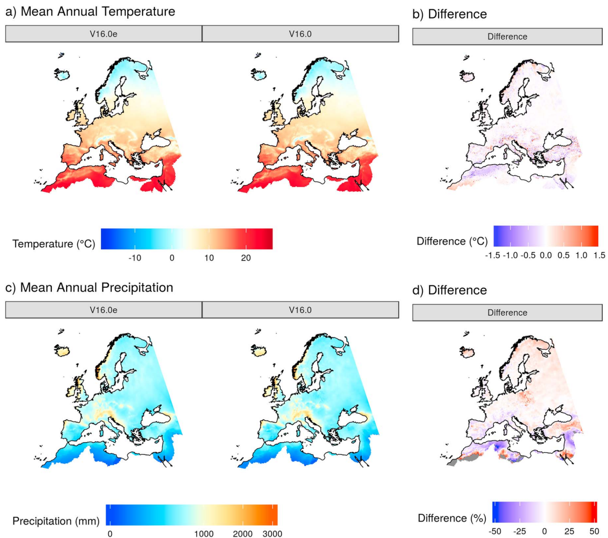
Figure 5. Climatology comparisons between E-OBS v16.0e and v16.0 for (a) mean annual temperature (tg) and (c) annual precipitation totals, calculated over the period 1981–2010. Indicated in (b) and (d) are the differences between the new and old E-OBS versions. In the case of precipitation (d) the difference is expressed as a proportion of mean precipitation totals from the old data set.
