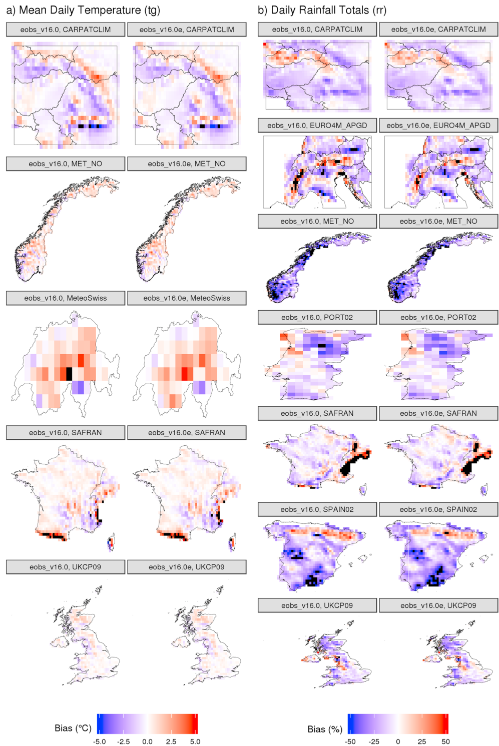
Figure 9. Annual climatological differences between E-OBS v16.0e and v16.0 compared to a selection of gridded data sets produced by NMS across Europe for tg (a) and rr (b). The annual averages are calculated over the period 1971–2010 and then the differences derived. In the case of precipitation the differences are expressed as a proportion of the NMS average totals. Grid box values beyond the respective color ranges are marked in black. NMS = National Meteorological Service.
