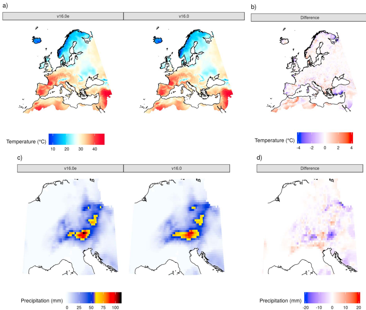
Figure 6. The gridded fields in E-OBS v16.0e and v16.0 for tx on 4 August 2003 (a) and rr on 1 June 2013 (c). The respective differences between the E-OBS versions are shown in (b) and (d).
