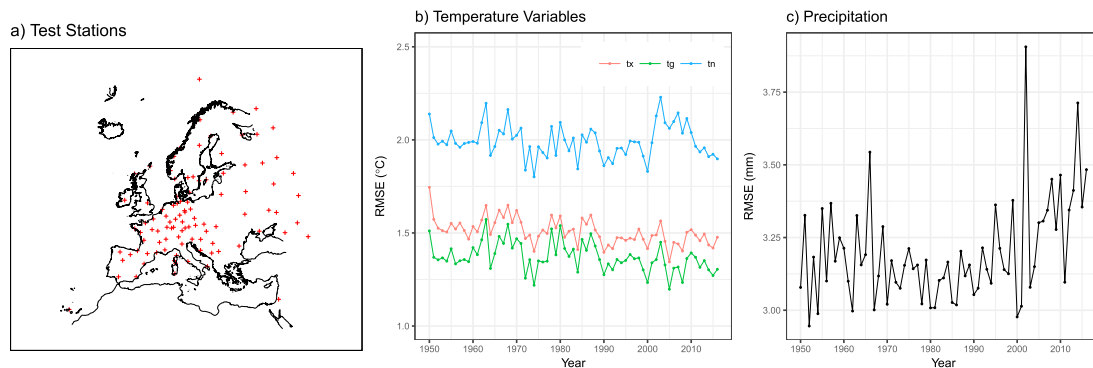
Figure 2. The locations of the 100 withheld test stations (a) and the yearly root-mean-square error (RMSE) values between interpolated values and recorded values at those stations for the temperature variables (b) and precipitation (c).
