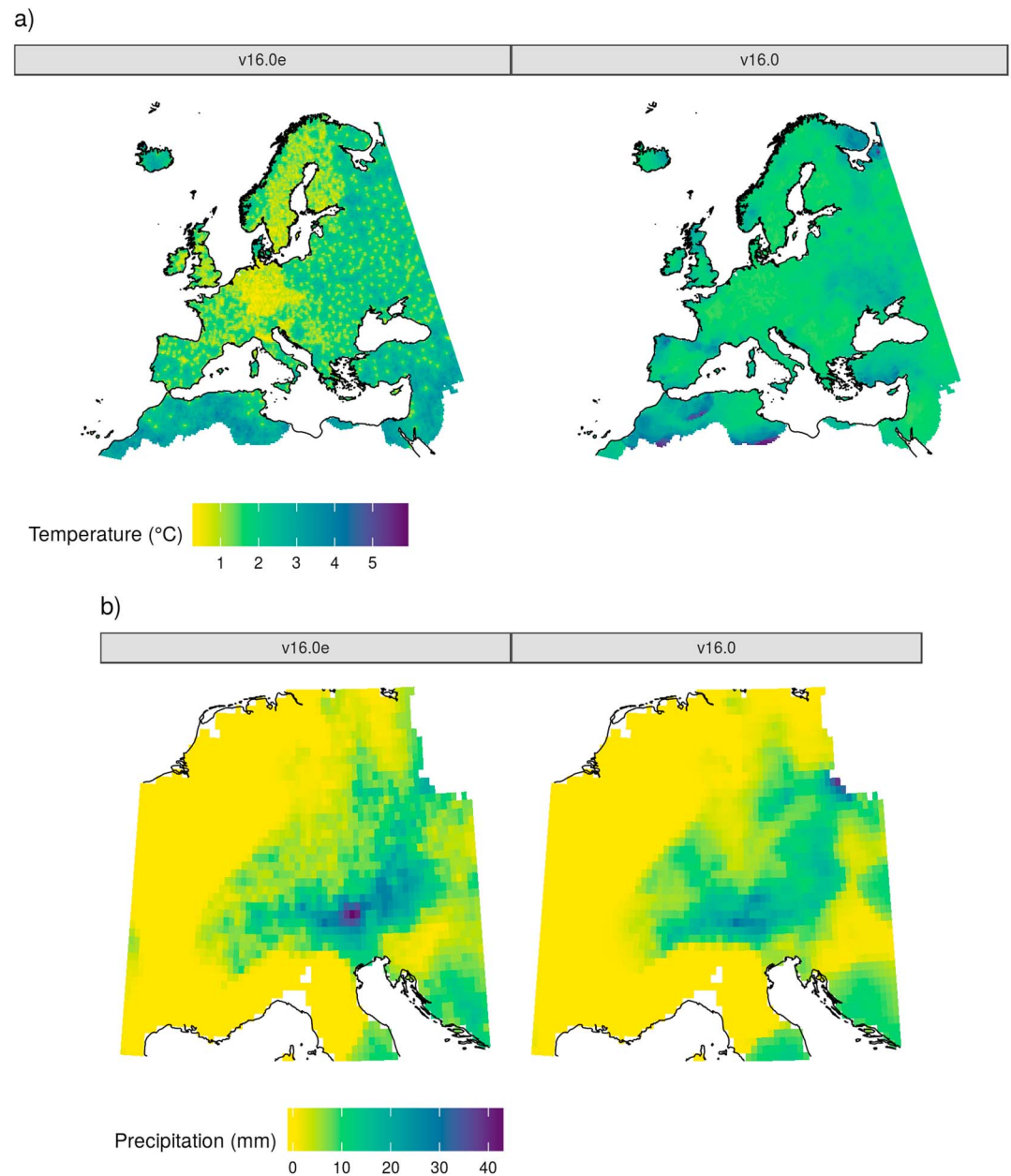
Figure 8. Uncertainty estimates in the tx gridded data for the 4 August 2003 event (a) and for the 1 June 2013 precipitation event (b).
