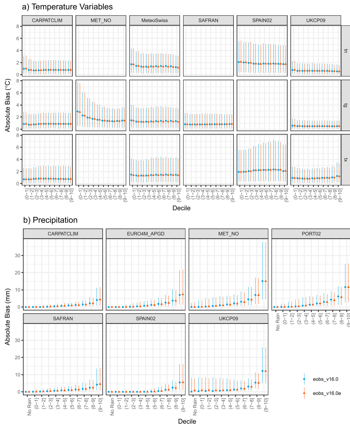
Figure 10. Absolute bias (E-OBS minus NMS data) in tg, tn, and tx (a) and rr (b) calculated from daily values over the period 1971–2010 grouped by decile determined by the NMS gridded data. The points indicate the median in each category, and the lines indicate the 10th–90th percentile. NMS = National Meteorological Service.
